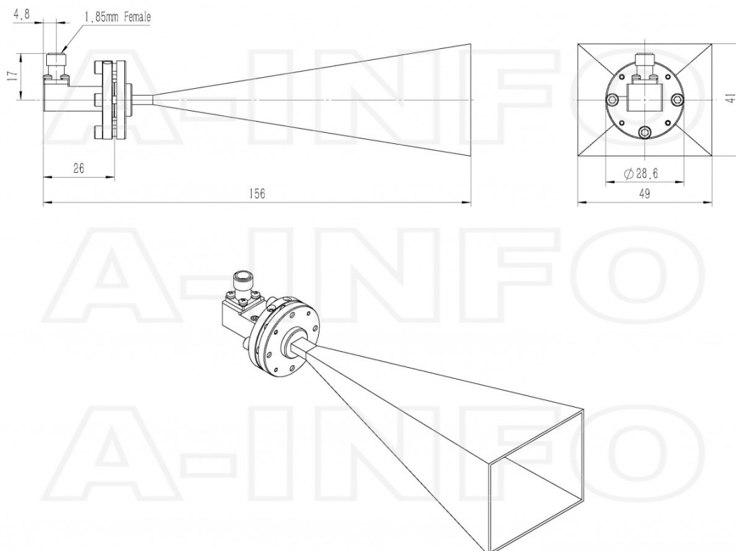
1.85mm-Female Output (P/N: LB-19-25-C-1.85F)
